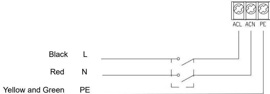
Relay Output (Optional)
